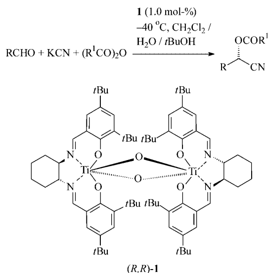
Scheme 1. Synthesis of cyanohydrin esters using catalyst 1 .
