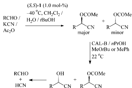
Scheme 2. Chemo-enzymatic synthesis of ( R )- O -acetylcyanohydrins.
